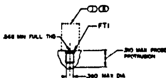
FUEL INLET TEMP FTI
